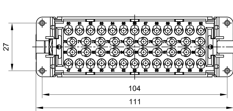
Panel cut out 面板开孔尺寸
